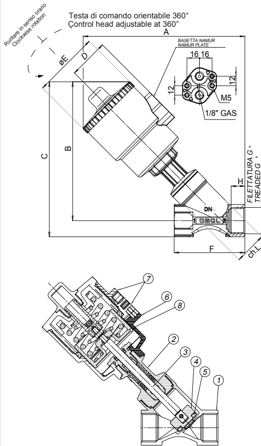
ZEUS - PN16 , NC , Screw BSP
