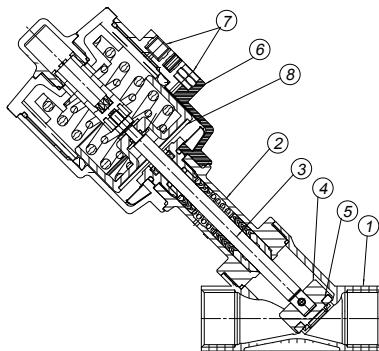
ARES - PN25 , NC , Screw BSP
